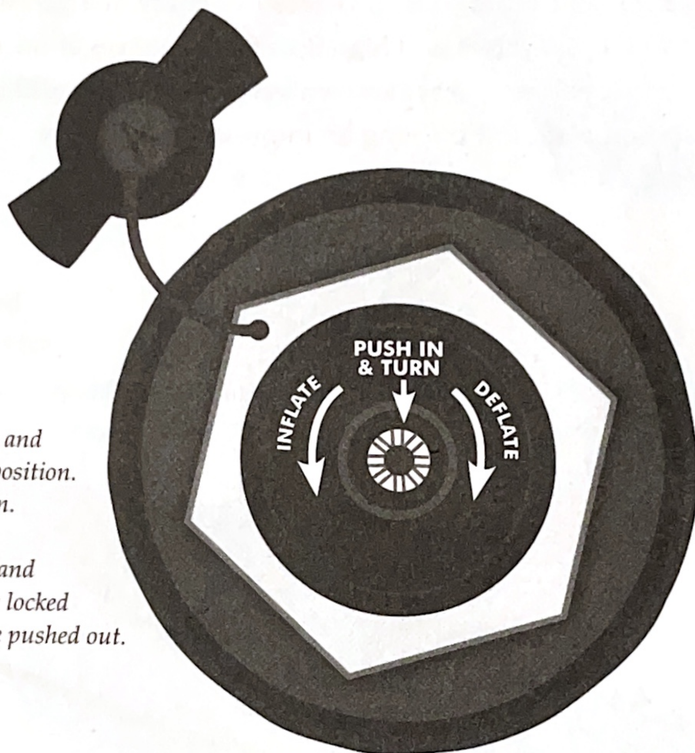
Figure 1. Inflate/Deflate Spring Valve
